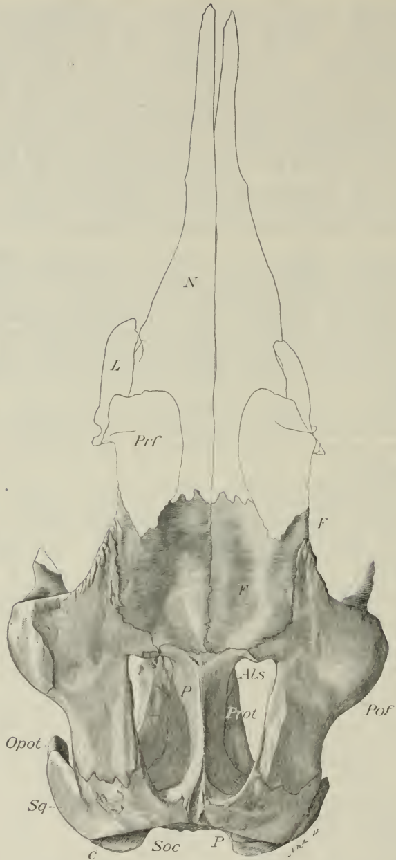
Figure 8. Cranium of Edmontosaurus , Cat. No. 2289; \frac{1}{2} natural size; superior aspect. Als , alisphenoid; F , frontal; L , lachrymal; N , nasal; Opot , opisthotic; P , parietal; Pof , post-frontal; Prf , prefrontal; Prot , proötic; Soc , supra-occipital; Sq , squamosal.
